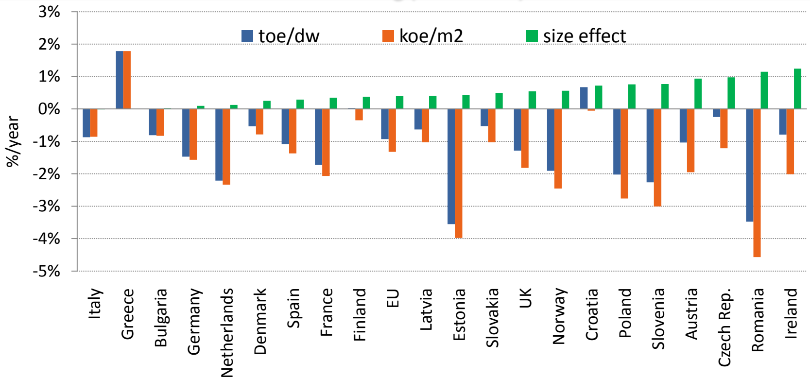
Average consumption per m 2 vs consumption per dwelling for household for space heating (1997-2008)
